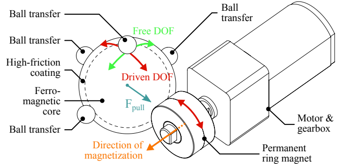
Fig. 1. Overview of our design. The ball wheel with ferromagnetic core is driven by a permanent ring magnet that acts as the drive roller. The magnet temporarily magnetizes the wheel, exerting a pull force and generating the necessary normal force. The wheel thus acquires one driven and one free DOF, kinematically equivalent to an omniwheel.
